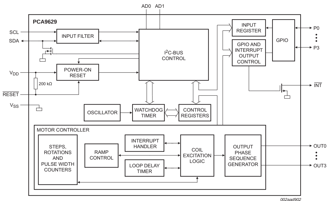
Fig 1. PCA9629 block diagram
